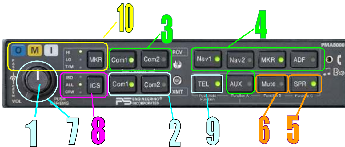
Figure 3-1 PMA8000B Operating Controls
